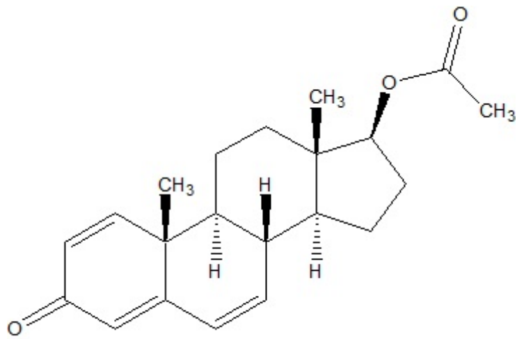
1,4,6-Androstatrien-17beta-ol-3-one acetate
